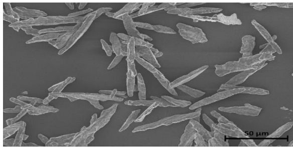
Figure 2. SEM Analysis of Struvite Crystals
