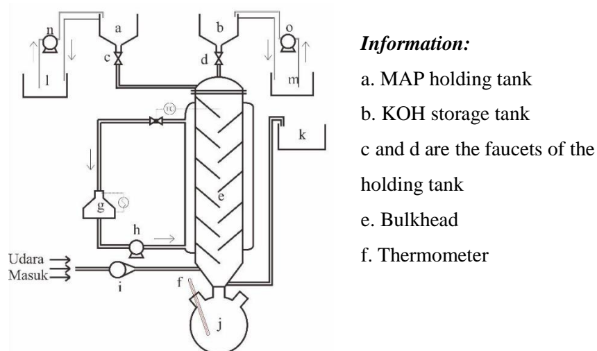
Figure 3. The series of bulkhead reactors
